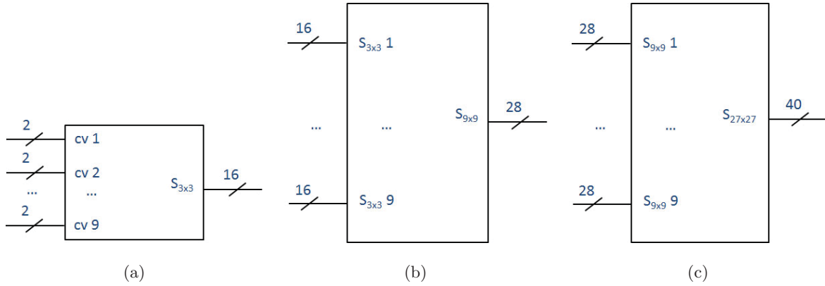
Fig. 9 Architectural blocks for: (a) 3x3 smoothing using cluster values ( cv 1- cv 9) from clustering operation, (b) 9x9 smoothing using results from nine 3x3 smoothing blocks ( S_{3x3} 1- S_{3x3} 9), and (c) 27x27 smoothing using results from nine 9x9 smoothing blocks ( S_{9x9} 1- S_{9x9} 9).
