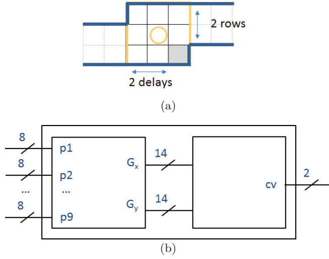
Fig. 8 For clustering block: (a) Number of registers necessary to parallelize the processing of the 3x3 window. The pixel in gray is the current pixel and the cluster direction is computed for the pixel indicated by a circle. (b) Architectural block where p1-p9 are 8-bit image pixels, G_x and G_y are gradient values coded in 14 bits, and cv is the resulting cluster value coded with 2 bits.
